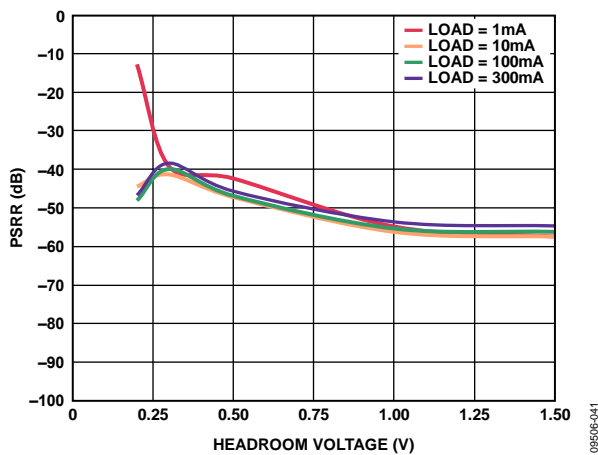
Figure 48. Power Supply Rejection Ratio vs. Headroom Voltage, 100 kHz, V_{OUT} = 5\text{ V}
