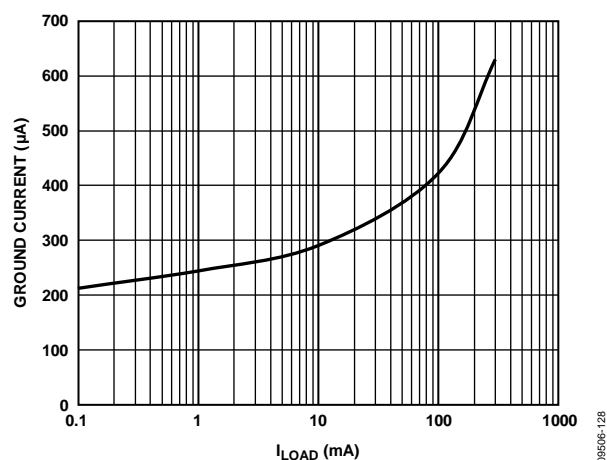
Figure 28. Ground Current vs. Load Current, V_{OUT} = 1.8\text{ V}
