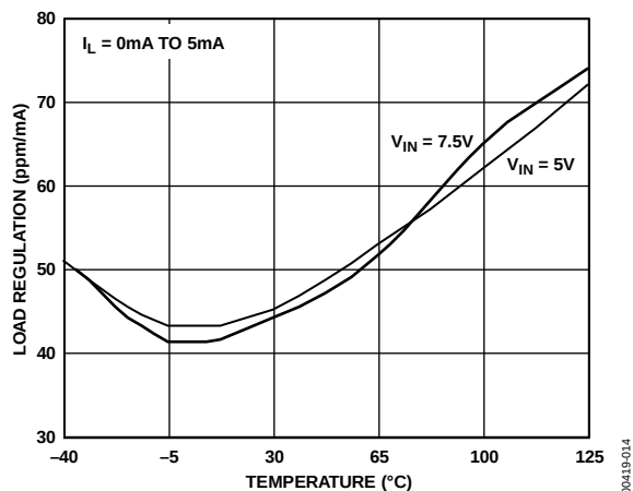
Figure 10. ADR395 Load Regulation vs. Temperature
