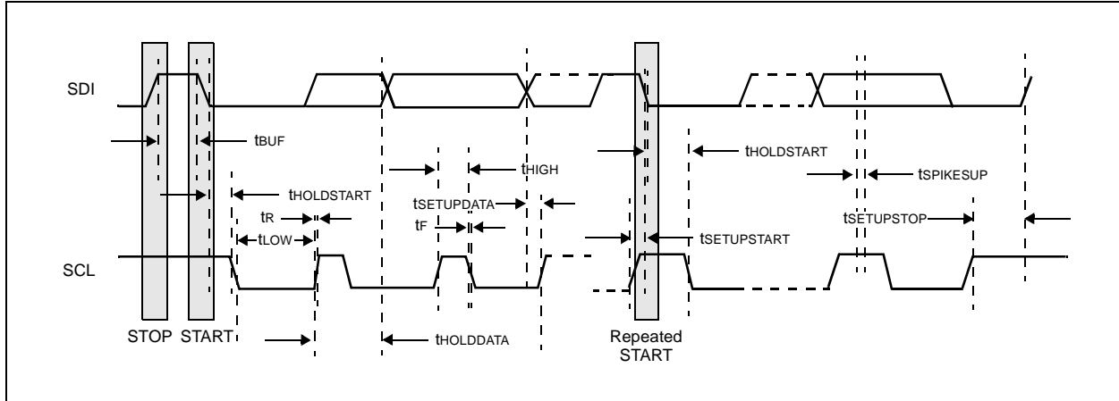
Figure 3. Timing Diagram
