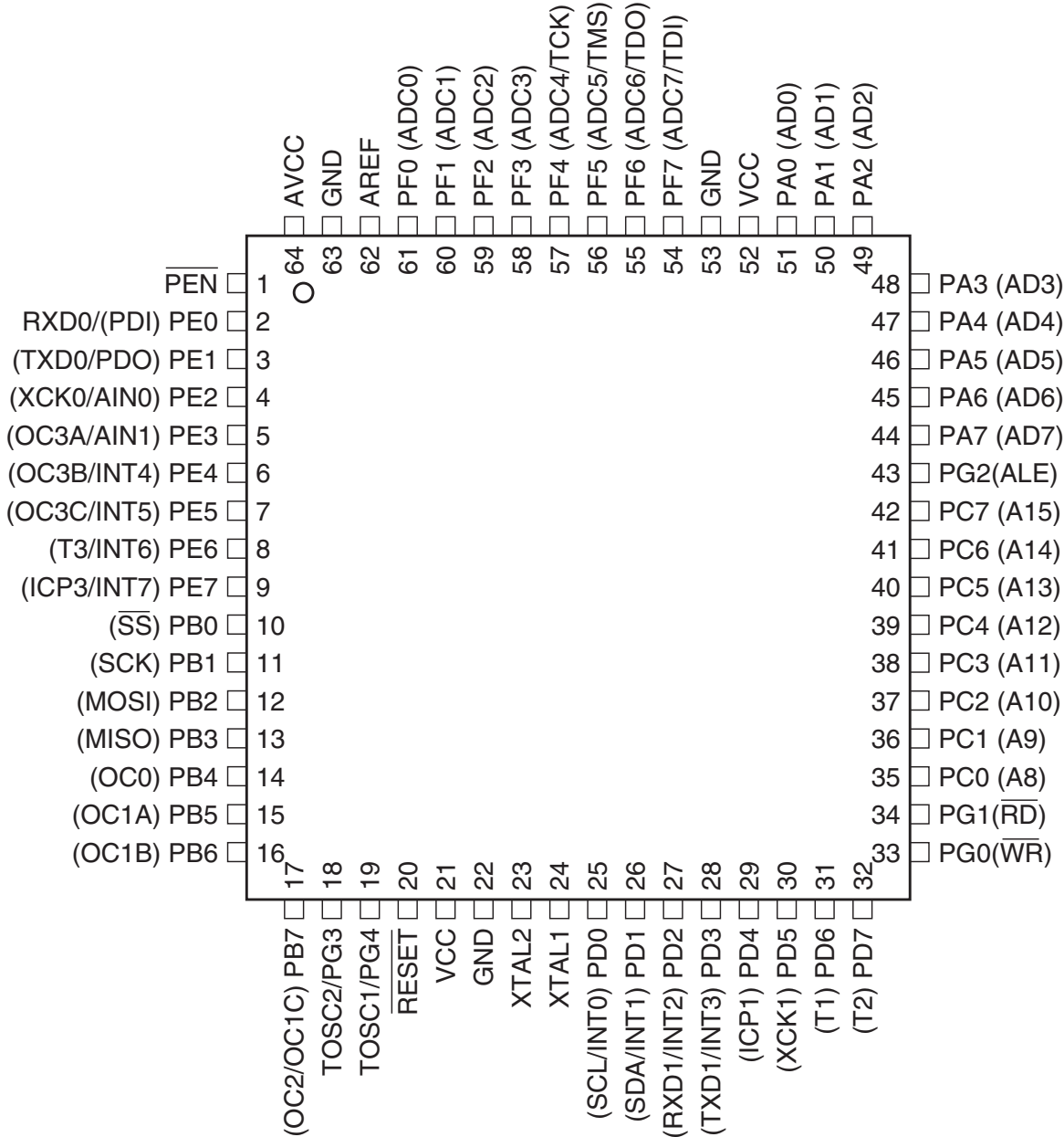
Figure 1-1. Pinout ATmega128A
