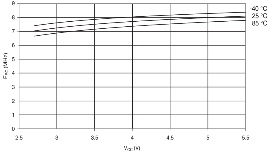
Figure 28-43. Calibrated 8MHz RC Oscillator Frequency vs. V CC
