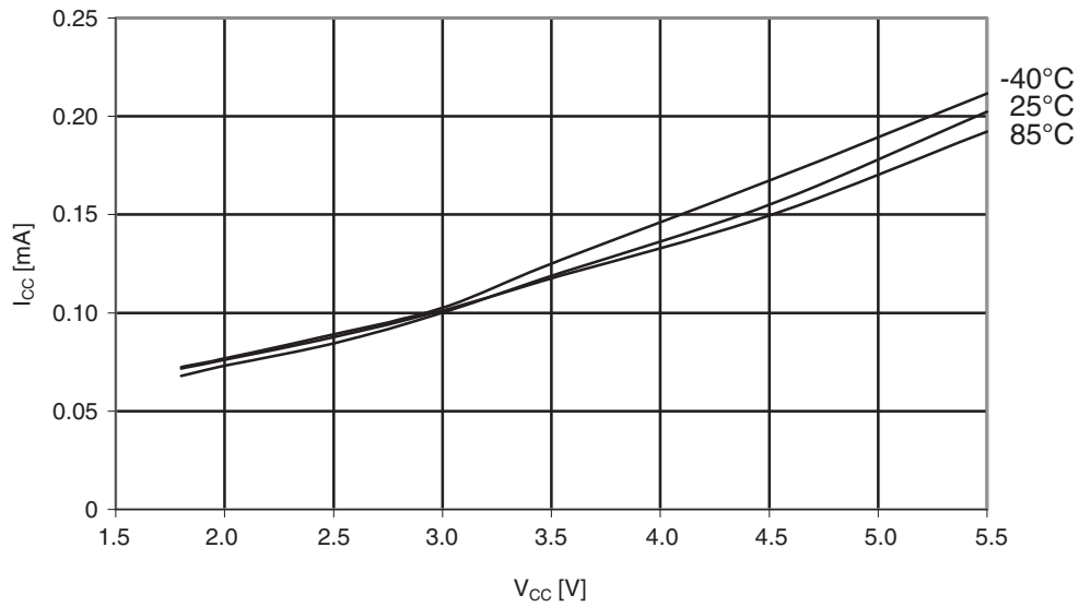
Figure 30-54. Atmel ATmega164PA: Active supply current vs. V_{CC} (internal RC oscillator, 128kHz).
