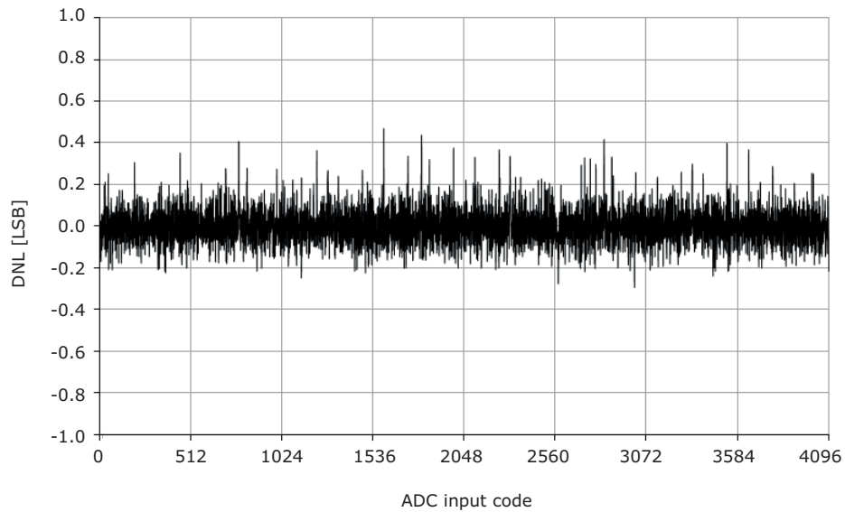
Figure 37-123. DNL error vs. input code.
