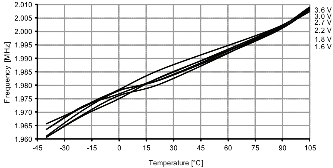
Figure 37-72. 2MHz internal oscillator frequency vs. temperature. DFLL enabled, from the 32.768kHz internal oscillator.
