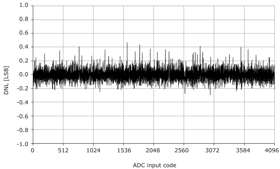
Figure 37-40. DNL error vs. input code.
