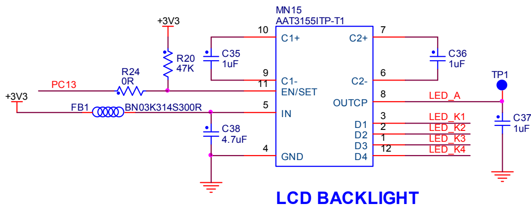
Figure 4-11. Backlight control.
