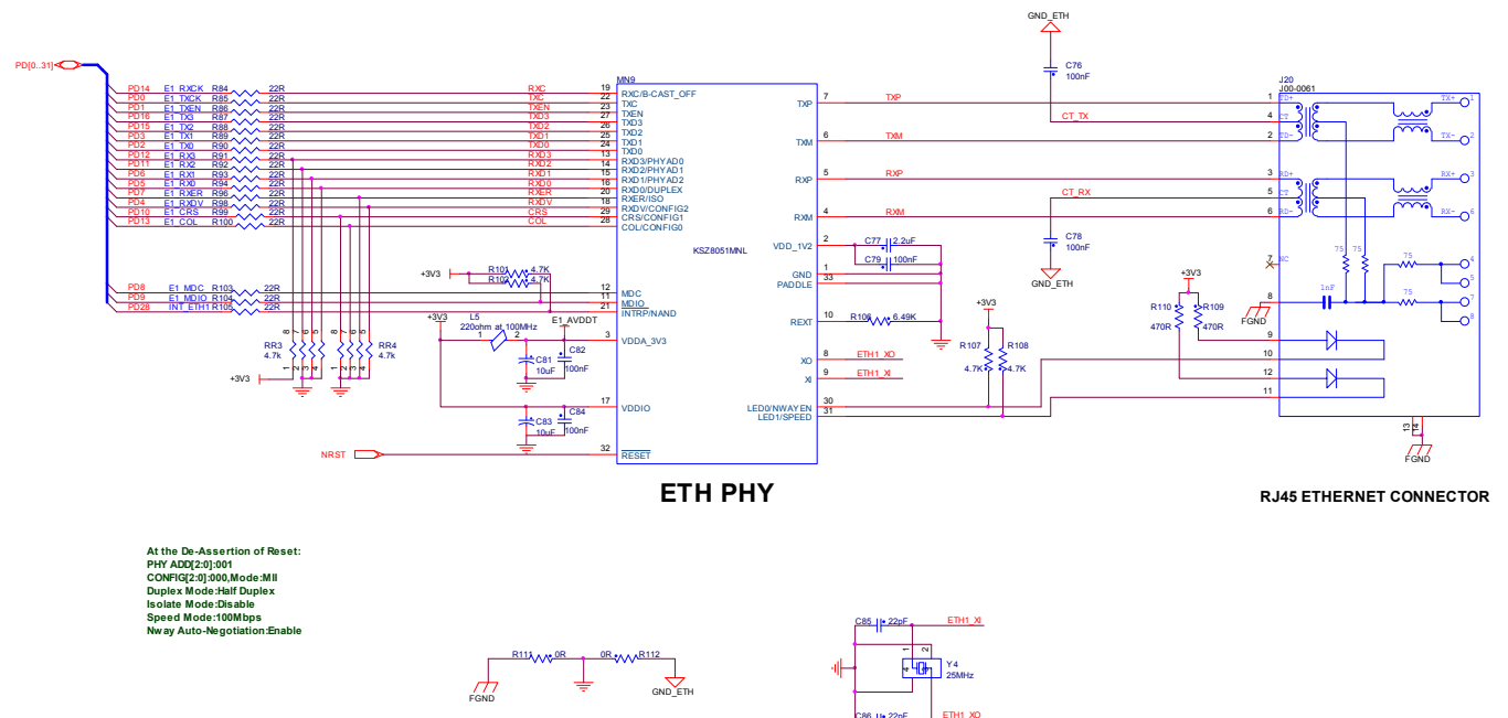
Figure 4-8. Ethernet block.
