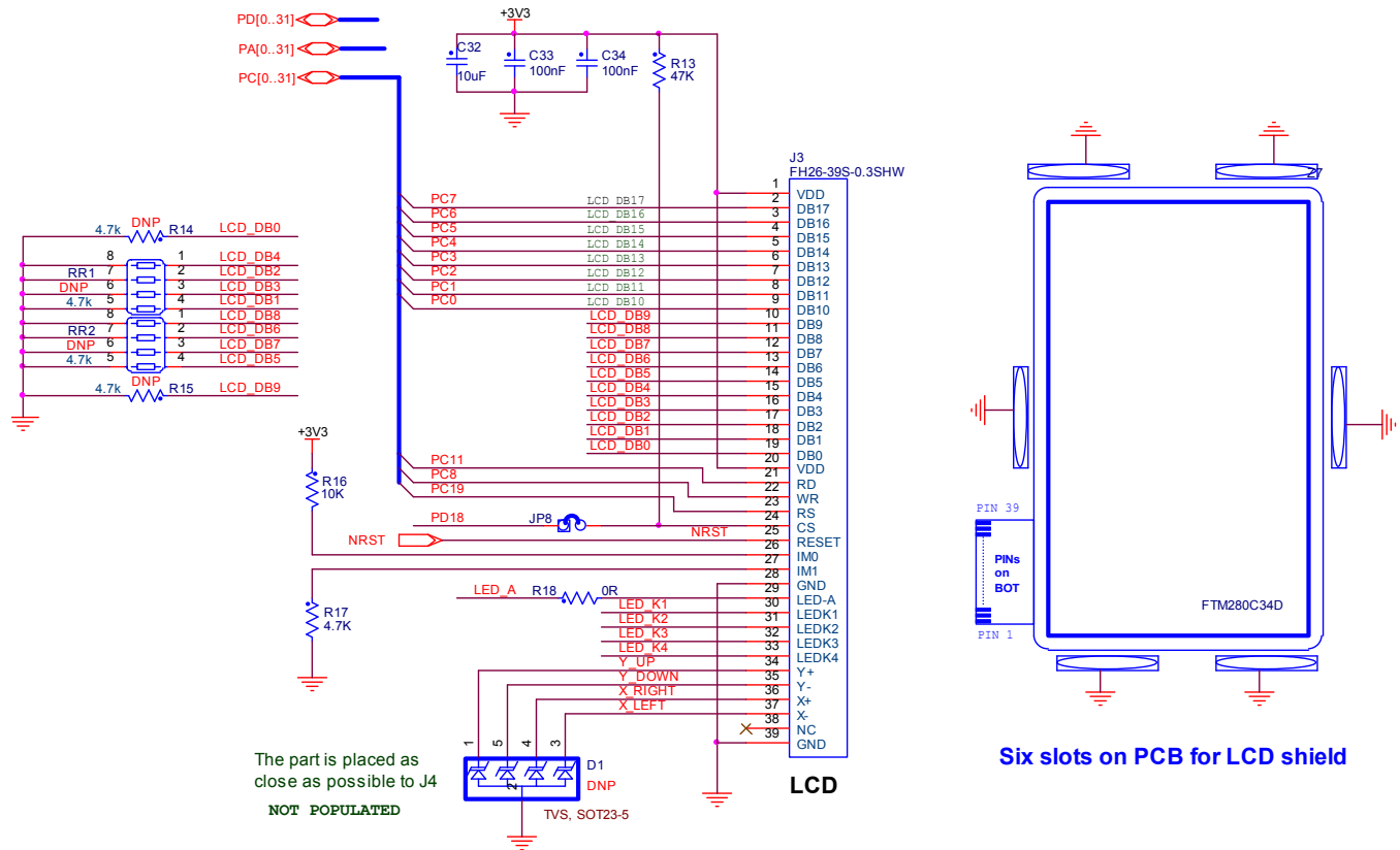
Figure 4-10. LCD block.
