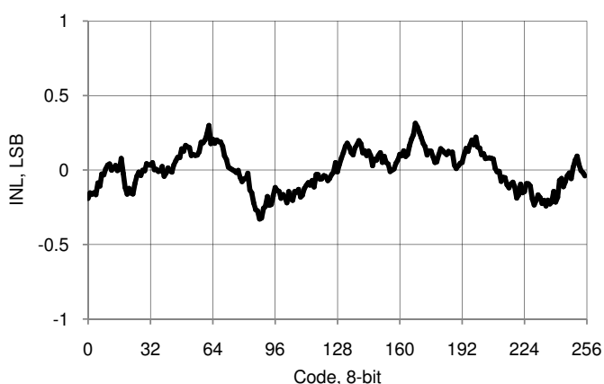
Figure 11-29. IDAC INL vs Input Code, Range = 255 \mu A, Sink Mode
