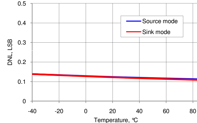
Figure 11-33. IDAC DNL vs Temperature, Range = 255 \mu A, Fast Mode
