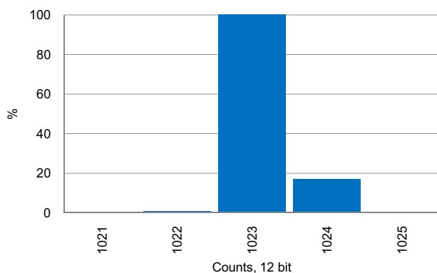
Figure 11-25. SAR ADC Noise Histogram, 100 kpsps, Internal Reference No Bypass
