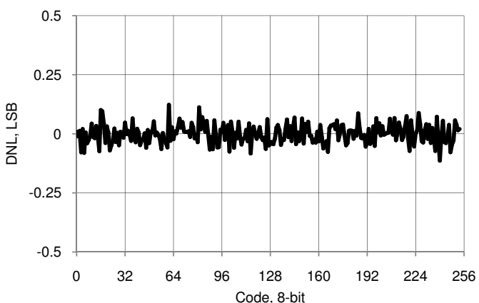
Figure 11-31. IDAC DNL vs Input Code, Range = 255 \mu A, Sink Mode
