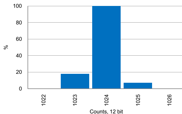
Figure 11-26. SAR ADC Noise Histogram, 1 msps, Internal Reference Bypassed
