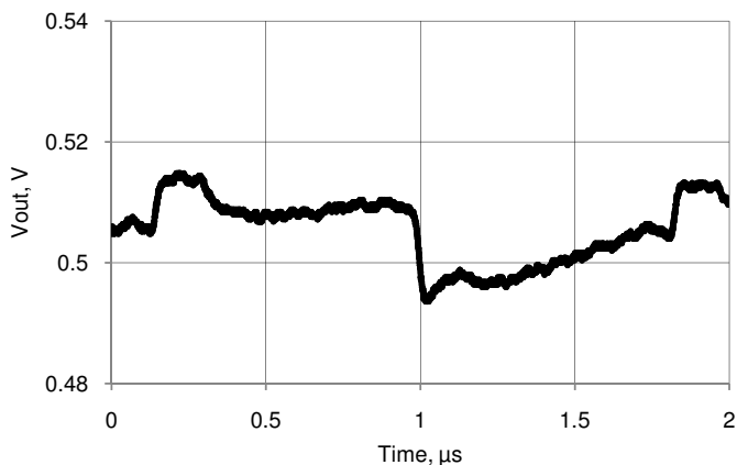
Figure 11-53. VDAC Voltage Noise, 1 V Mode, Fast Mode, V_{DDA} = 5 V
