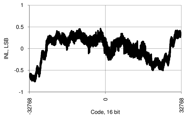
Figure 11-33. Delta-sigma ADC INL vs Output Code, 16-bit, 48 ksps, 25 °C V_{DDA} = 3.3 V
