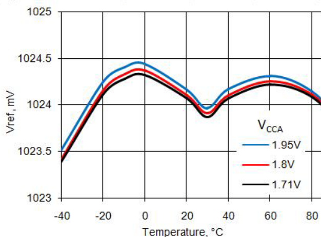
Figure 11-34. Vref vs Temperature
