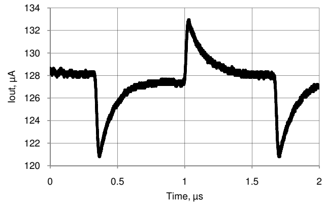
Figure 11-52. IDAC Glitch Response, Codes 0x7F - 0x80, 255 \mu A Mode, Source Mode, Fast Mode, V_{DDA} = 5 V
