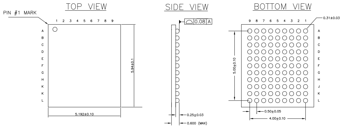
Figure 2. WLCSP Package (5.192 × 5.940 × 0.6 mm)
