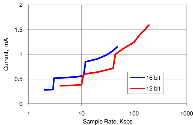
Figure 11-28. Delta-sigma ADC IDD vs sps, Range = \pm 1.024 V, Continuous Sample Mode, Input Buffer Bypassed
