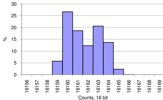
Figure 11-30. Delta-sigma ADC Noise Histogram, 1000 Samples, 16-bit, 48 ksps, Ext Ref, V_{IN} = V_{REF}/2 , Range = \pm 1.024 V
