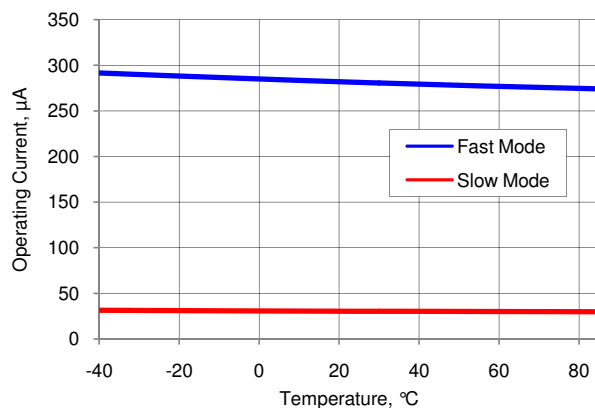
Figure 11-49. IDAC Operating Current vs Temperature, Range = 255 \mu A, Code = 0, Source Mode
