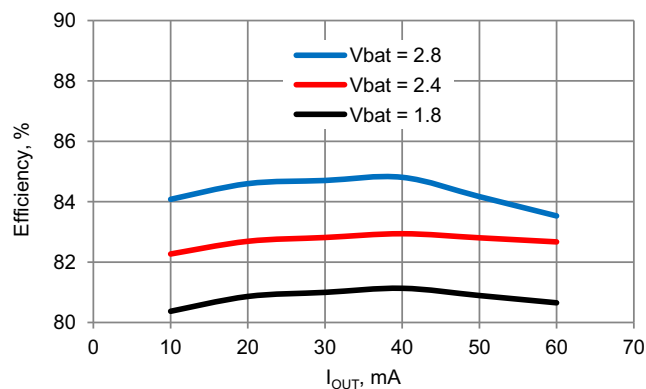
Figure 11-8. Efficiency vs I_{\text{OUT}} V_{\text{BOOST}} = 3.3 \text{ V} , L_{\text{BOOST}} = 10 \mu\text{H} [28]
