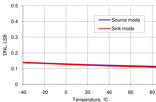
Figure 11-46. IDAC DNL vs Temperature, Range = 255 \mu A, Fast Mode
