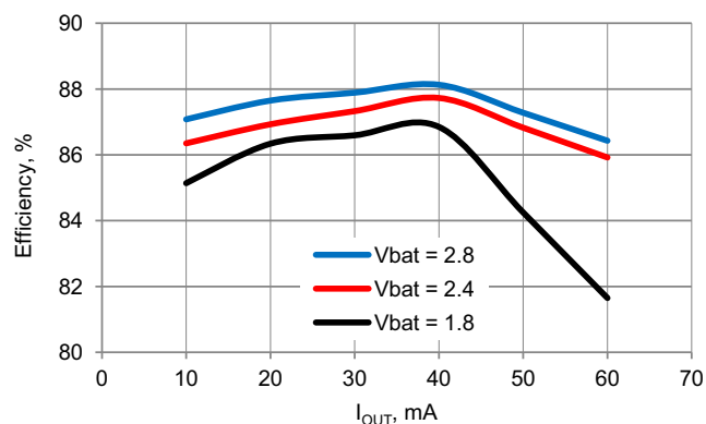
Figure 11-9. Efficiency vs I_{\text{OUT}} V_{\text{BOOST}} = 3.3 \text{ V} , L_{\text{BOOST}} = 22 \mu\text{H} [28]
