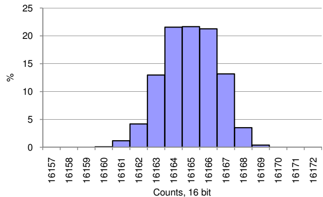
Figure 11-31. Delta-sigma ADC Noise Histogram, 1000 Samples, 16-bit, 48 ksps, Int Ref, V_{IN} = V_{REF}/2 , Range = \pm 1.024 V
