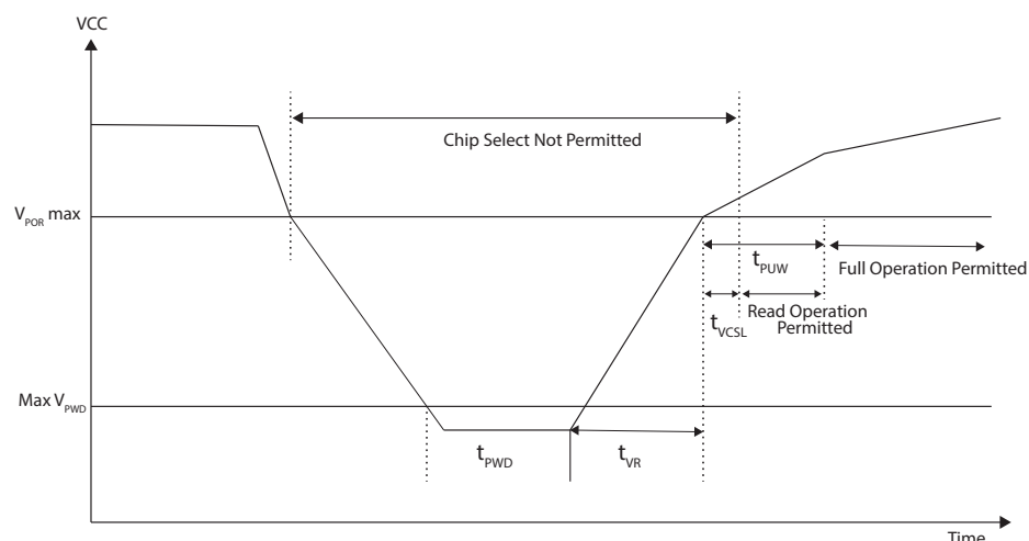
Figure 16-1. Power-Up Timing
