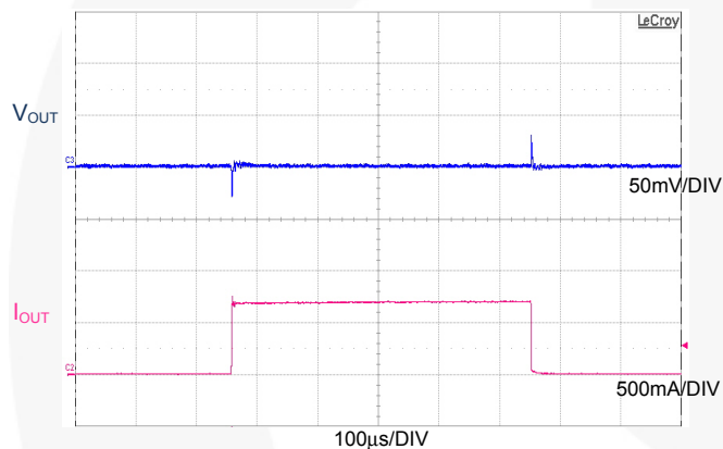
Figure 19. Load Transient in PWM Mode, V_{IN} = 3.8\text{ V} , V_{OUT} = 3.0\text{ V} , I_{OUT} = 0\text{ mA} to 700\text{ mA} , 10\text{ }\mu\text{s} Edge
