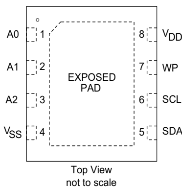
Figure 2. 8-pin TDFN pinout
