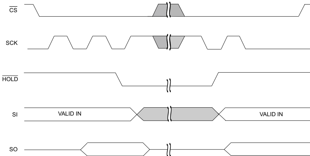
Figure 13. \overline{HOLD} Operation [2]
