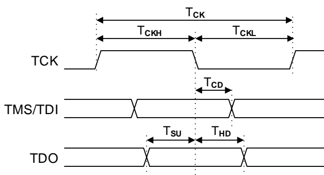
Figure 12. Timing diagram.
