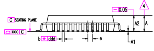
SIDE VIEW 2
