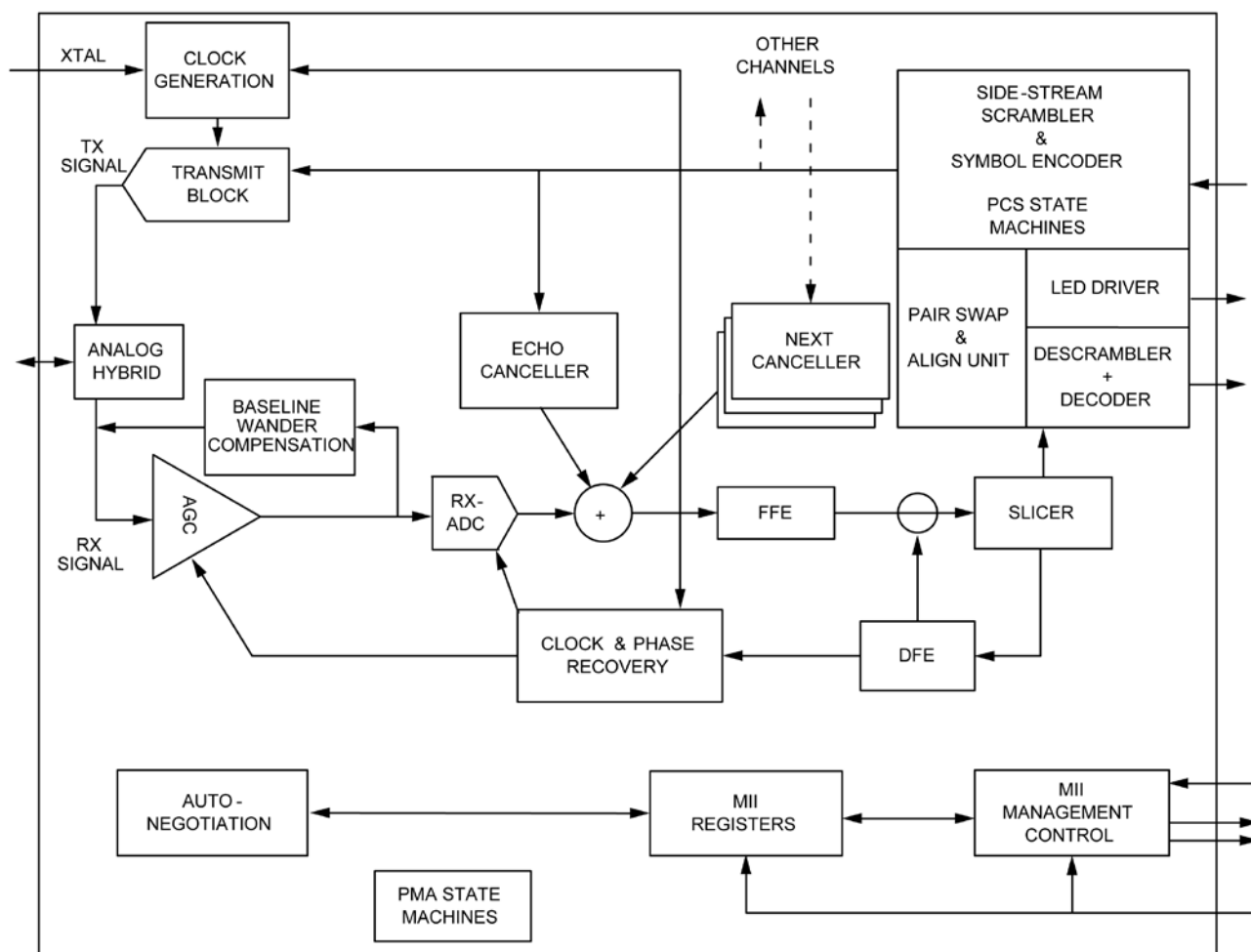
Figure 2. KSZ9031MNX 1000Base-T Block Diagram – Single Channel
