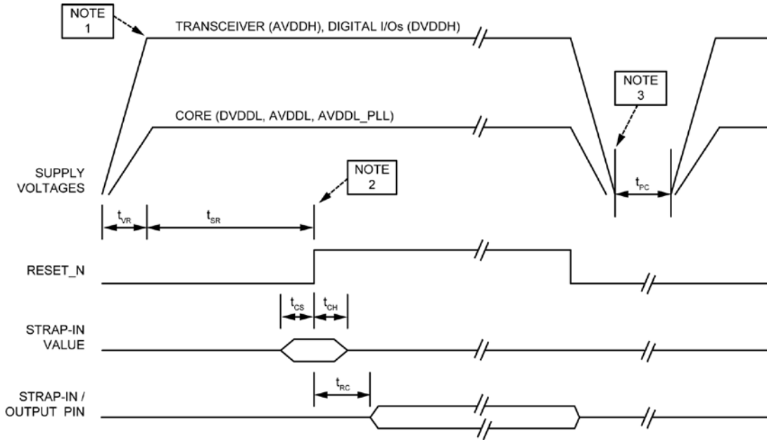
Figure 19. Power-Up/Power-Down/Reset Timing
