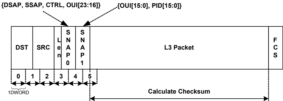
Figure 3.7 Ethernet Frame with Length Field and SNAP Header
