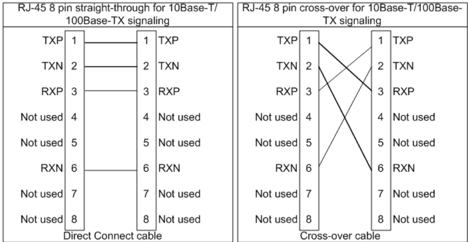
Figure 4.3 Direct cable connection vs. Cross-over cable connection.
