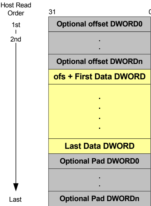
Figure 3.20 RX Packet Format
