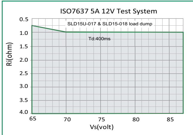
Figure 7 - SOA Chart
