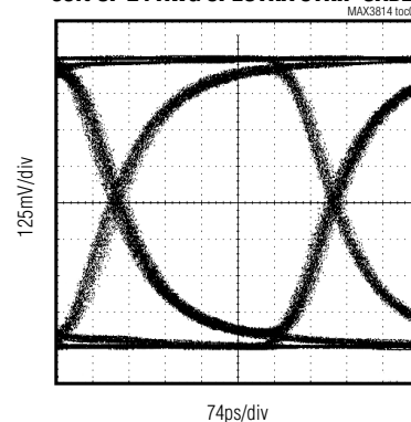
MAX3814 OUTPUT: 2.25Gbps DATA AFTER 33ft OF 24 AWG SPECTRA STRIP CABLE
