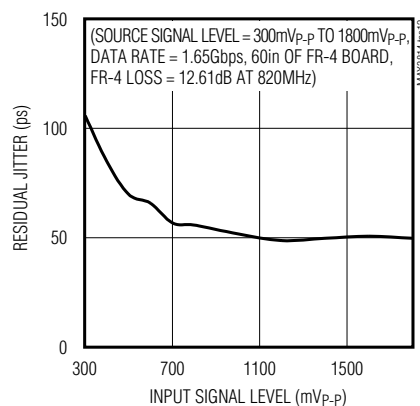
RESIDUAL JITTER
