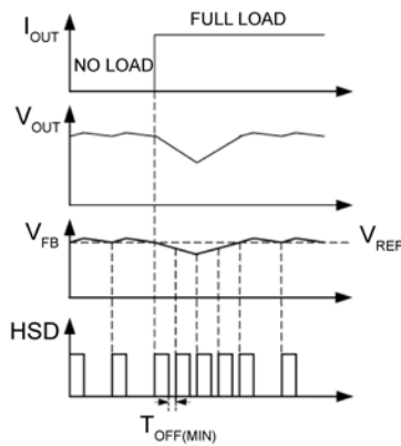
Figure 3. MIC24056 Load Transient Response
