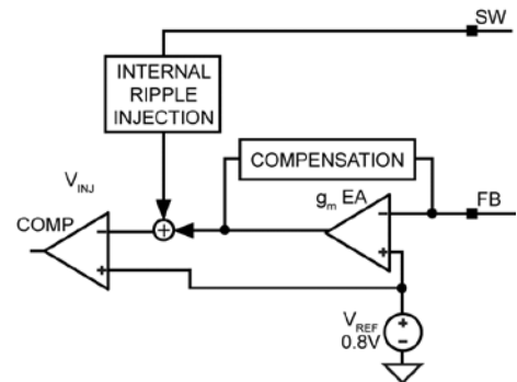
Figure 10. Internal Ripple Injection
