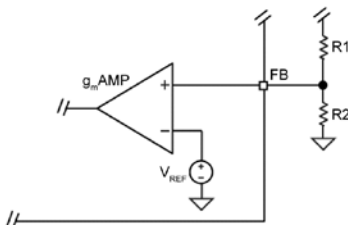
Figure 9. Voltage-Divider Configuration
