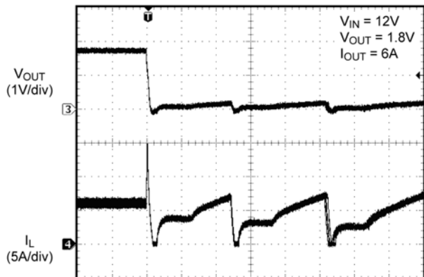
Short Circuit
