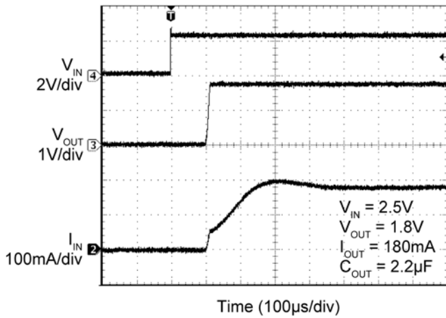
Inrush Current, C_{OUT} = 2.2\mu F
