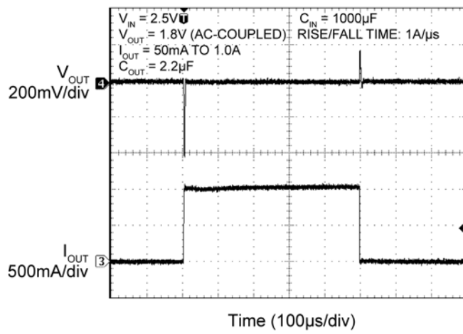
Fast Load Transient Response
