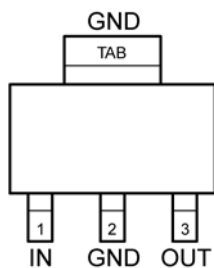
SOT-223 (S) MIC371x0-1.8 (Fixed)
