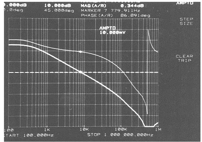
Figure 3b. 1.8V/2A Bode Plot ( \theta margin = 87°)
