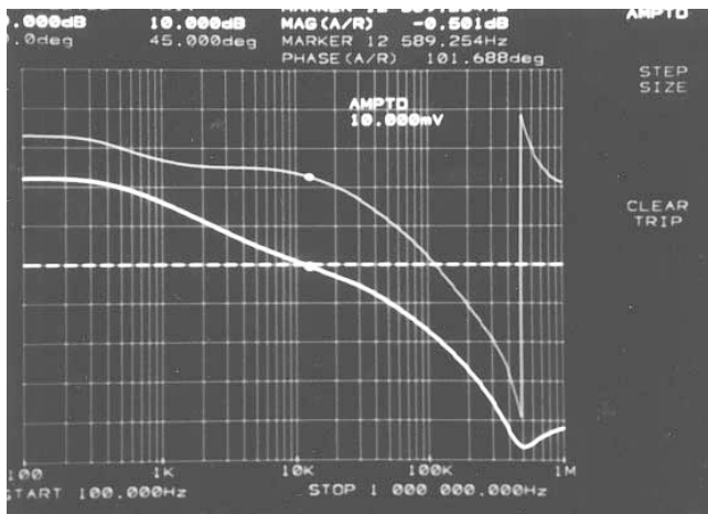
Figure 3a. 1.8V/1A Bode Plot ( \theta margin = 102°)
