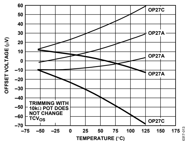
Figure 13. Offset Voltage Drift of Five Representative Units vs. Temperature
