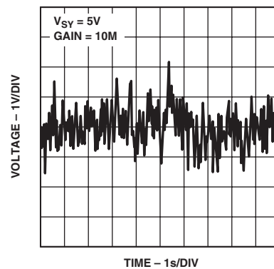
TPC 36. 0.1 Hz to 10 Hz Input Voltage Noise
