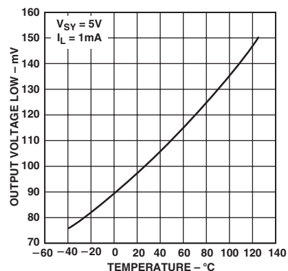
TPC 45. Output Voltage Low vs. Temperature
