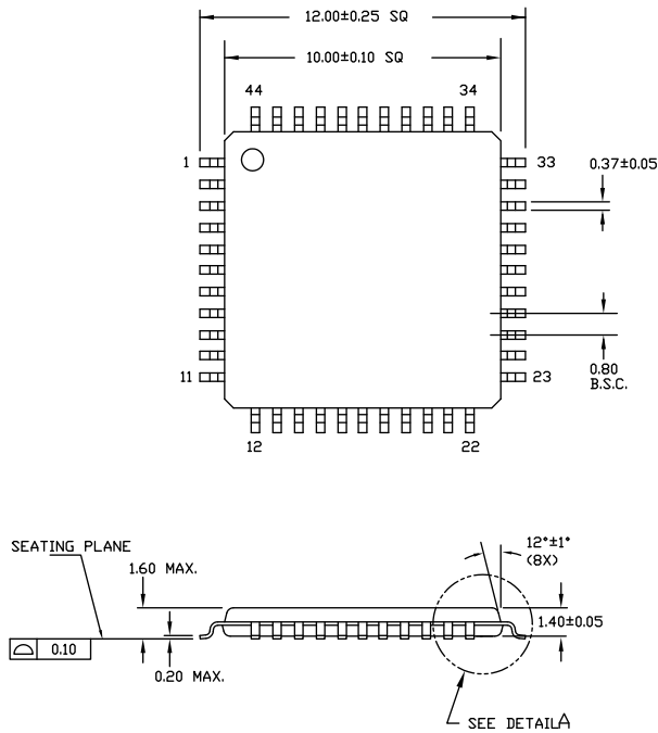
Figure 17. 44-pin TQFP Package Outline
