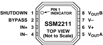
Figure 3. 8-Lead LFCSP_VD Pin Configuration (CP-8-2)
