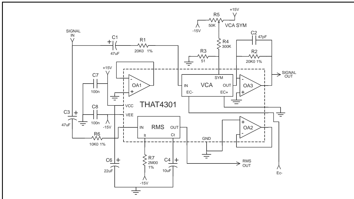
Figure 2. VCA and RMS detector test circuit
