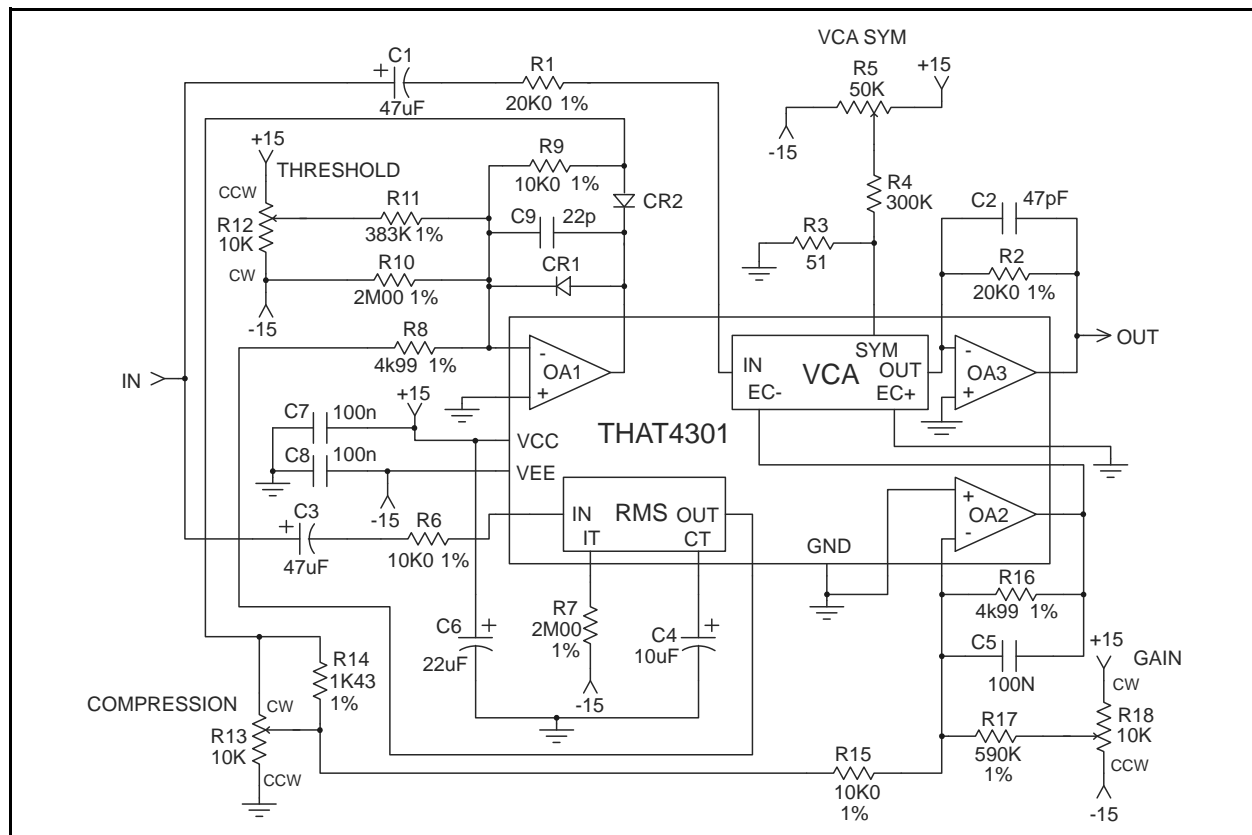
Figure 12. Typical Compressor/Limiter Application Circuit
