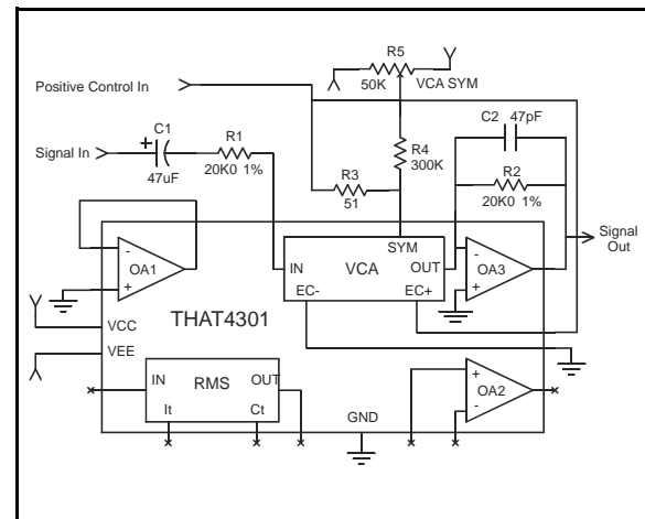
Figure 11. Driving the VCA via the Positive Control Port
