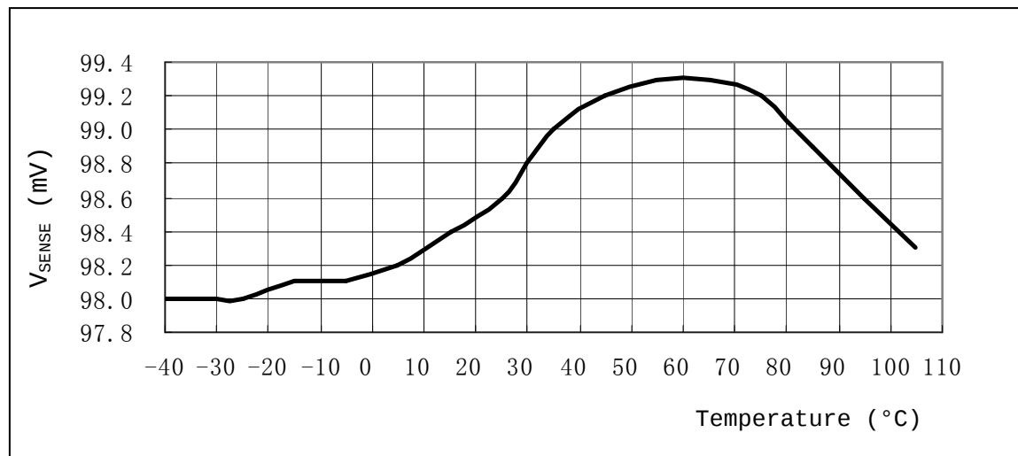
Figure 1.7 Sense Voltage vs. Operating Temperature ( R_s=0.10\Omega , L_1=47\mu\text{H} , V_{IN} = 40\text{ V} )
