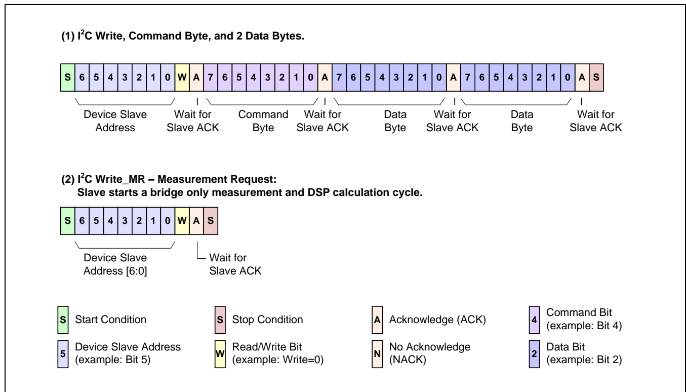
Figure 3.9 I 2 C TM Measurement Packet Writes
