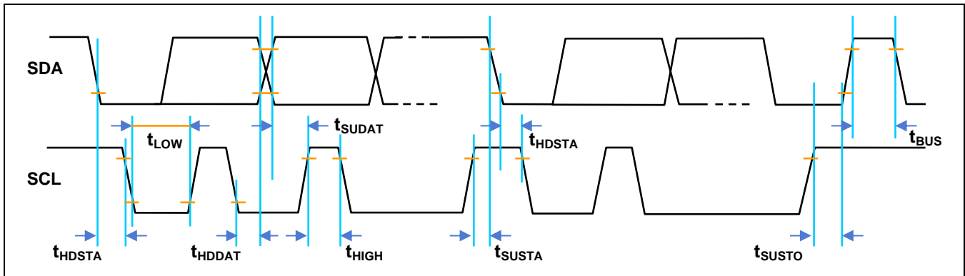
Figure 2.4 I 2 C TM Timing Diagram
