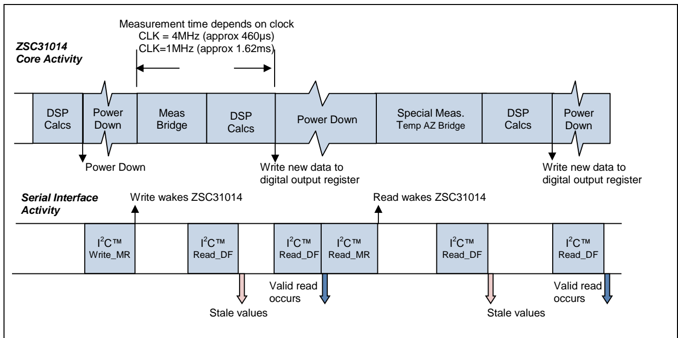
Figure 3.5 Sequence during Sleep Mode Using an I 2 C TM Write_MR to Wake Up (Typical Timing Values ** )
