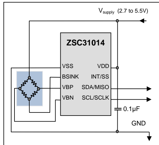
Figure 4.1 Example 1 Circuit Diagram: Bsink Option and Internal Temperature Correction and I 2 C TM Output
