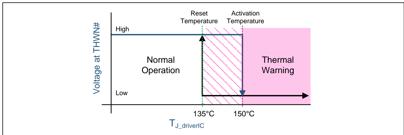
Figure 2.3 THWN# Operation
