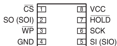
Figure 2-1. 8-SOIC (Top View)
