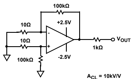
FIGURE 39. LONG TERM DRIFT TEST CIRCUIT
