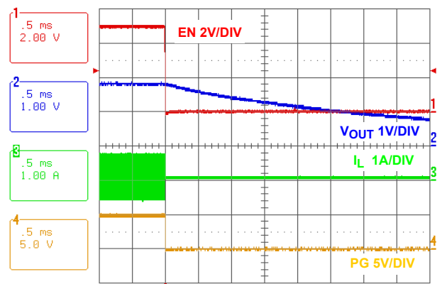
FIGURE 25. SOFT-DISCHARGE SHUTDOWN
