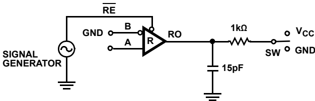
FIGURE 7. RECEIVER PROPAGATION DELAY AND DATA RATE
