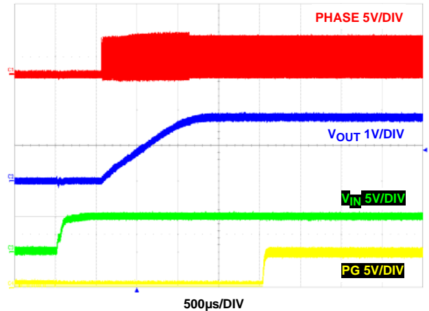
FIGURE 32. START-UP V_{\text{IN}} AT NO LOAD (PWM)
