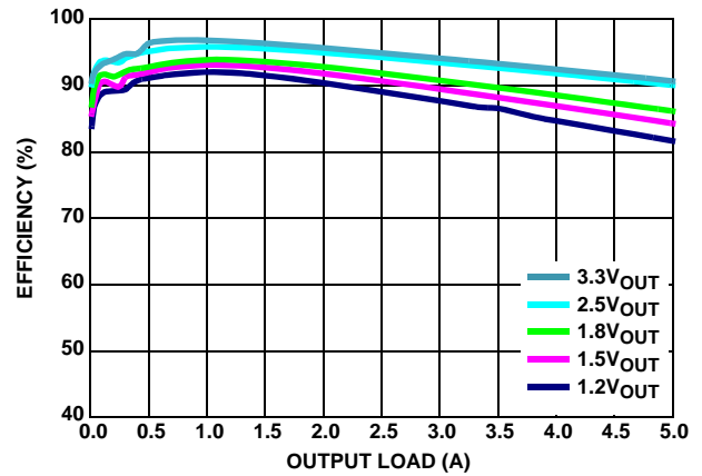
FIGURE 7. EFFICIENCY vs LOAD (1MHz 5V V_{IN} PFM)
