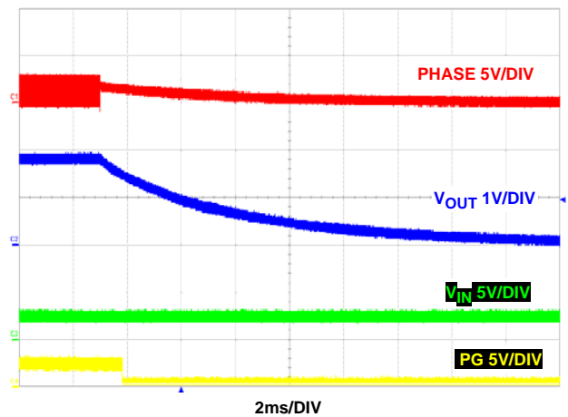
FIGURE 34. SHUTDOWN V_{\text{IN}} AT NO LOAD (PWM)
