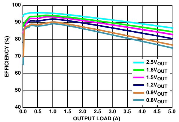
FIGURE 9. EFFICIENCY vs LOAD (2MHz 3.3V V_{IN} PFM)
