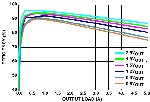
FIGURE 8. EFFICIENCY vs LOAD (2MHz 3.3V V_{IN} PWM)
