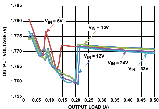
FIGURE 16. V_{OUT} REGULATION vs LOAD, PFM, V_{OUT} = 1.8V
