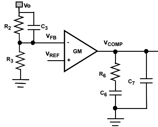
FIGURE 61. TYPE II COMPENSATOR
