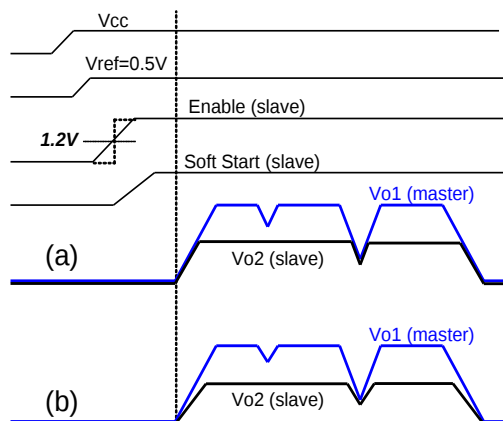
Figure 13: Typical waveforms for sequencing mode of operation: (a) simultaneous, (b) ratiometric
