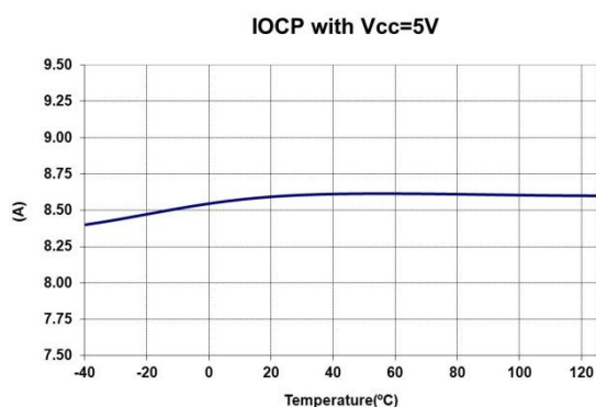
With an External 5V Vcc Voltage
