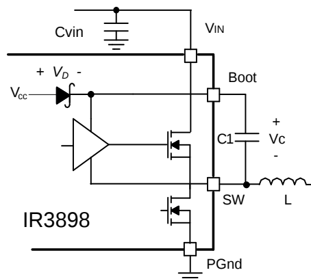
Figure 24: Bootstrap circuit to generate Vc voltage
