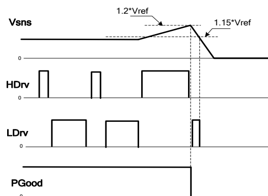
Figure 18c: Timing Diagram for OVP in non-tracking mode
