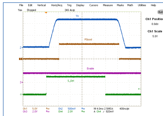
Figure 44: Start/Stop using S-ctrl pin Ch1-PGood,Ch2:Vout;Ch3-EN.Ch4-S-Ctrl
