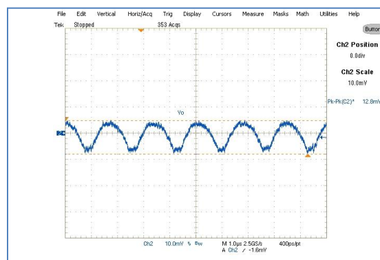
Figure 35: Output Voltage Ripple 6A Load Ch2: V_o
