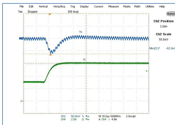
Figure 40: Transient Response, 3 to 6A step at 2.5A/µSec slew rate Ch2:V o , Ch4:I out (2A/Div)
