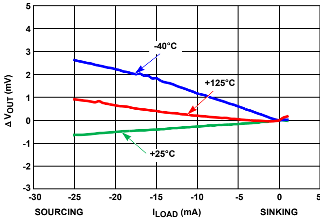
FIGURE 59. LOAD REGULATION OVER-TEMPERATURE
