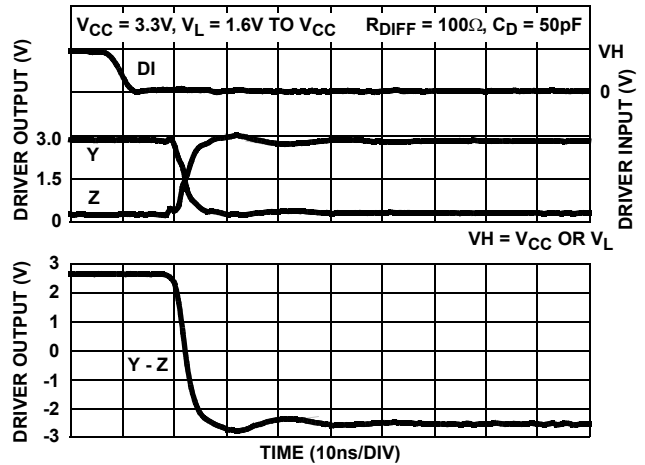
FIGURE 28. DRIVER WAVEFORMS, HIGH TO LOW (ISL32172E, ISL32174E, ISL32179E)
