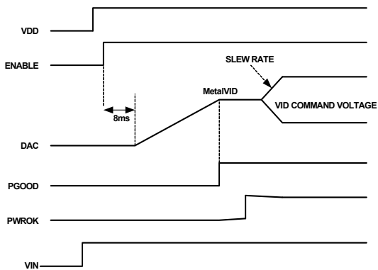
FIGURE 13. TYPICAL SOFT-START WAVEFORMS
