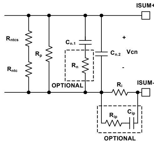
FIGURE 26. OPTIONAL CIRCUITS FOR RING-BACK REDUCTION
