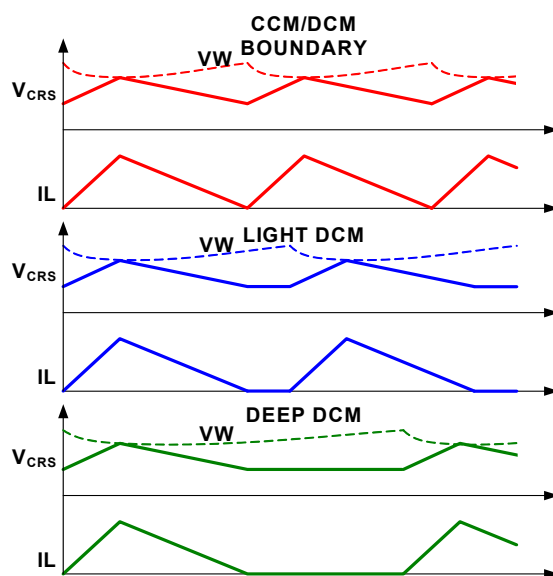
FIGURE 11. PERIOD STRETCHING
