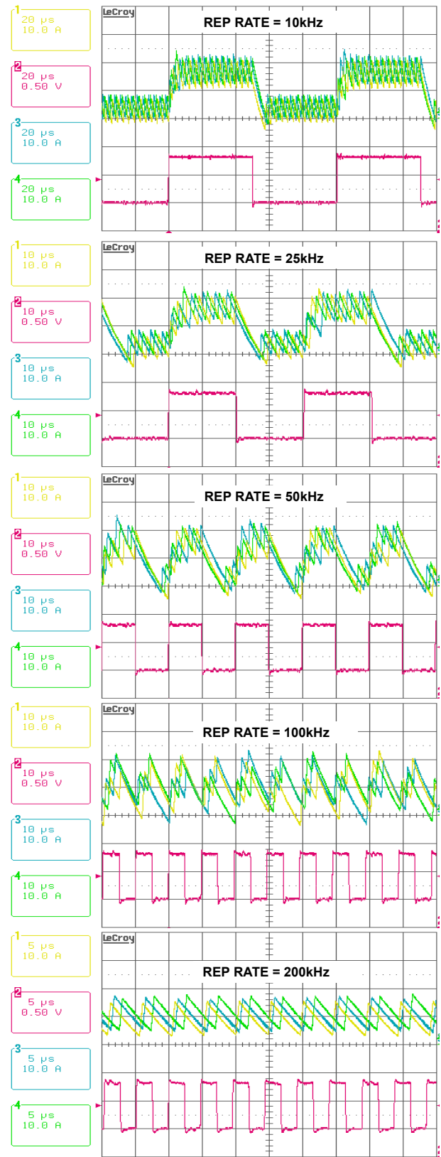
FIGURE 17. CURRENT BALANCING DURING DYNAMIC OPERATION. CH1: I L1 , CH2: I LOAD , CH3: I L2 , CH4: I L3
