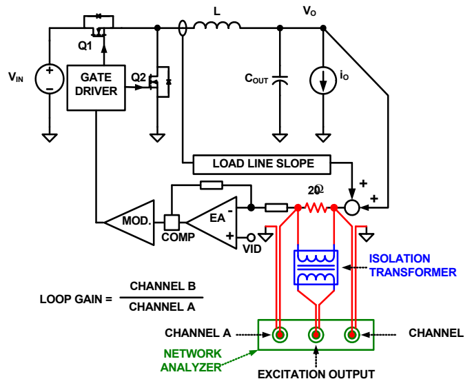
FIGURE 29. LOOP GAIN T1(s) MEASUREMENT SET UP
