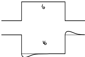
FIGURE 23. LOAD TRANSIENT RESPONSE WHEN C_n IS TOO SMALL
