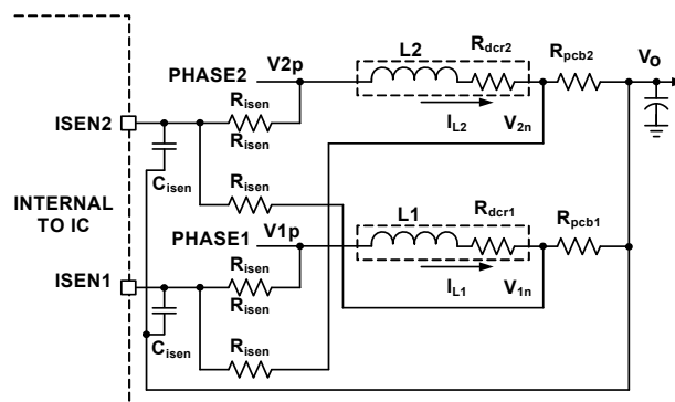
FIGURE 16. DIFFERENTIAL-SENSING CURRENT BALANCING CIRCUIT
