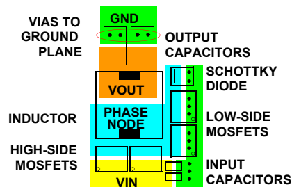
FIGURE 32. TYPICAL POWER COMPONENT PLACEMENT
