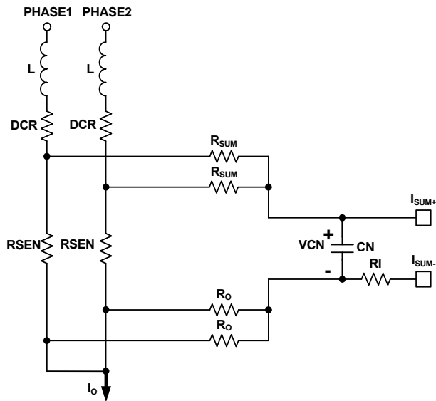
FIGURE 27. RESISTOR CURRENT-SENSING NETWORK
