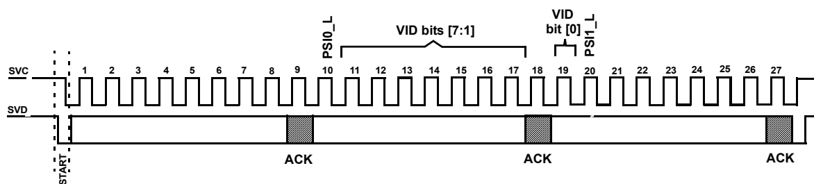
FIGURE 18. SVD PACKET STRUCTURE
