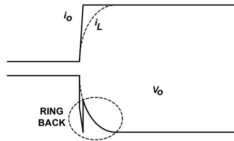
FIGURE 25. OUTPUT VOLTAGE RING-BACK PROBLEM
