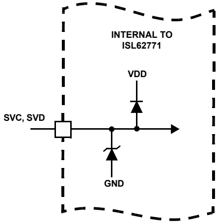
FIGURE 20. PROTECTION DEVICES ON THE SVC AND SVD PINS
