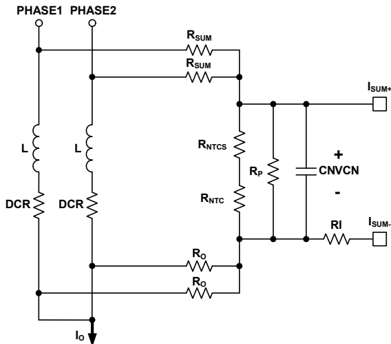
FIGURE 21. DCR CURRENT-SENSING NETWORK
