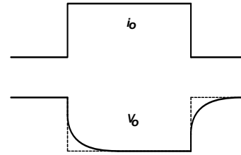
FIGURE 24. LOAD TRANSIENT RESPONSE WHEN C_n IS TOO LARGE
