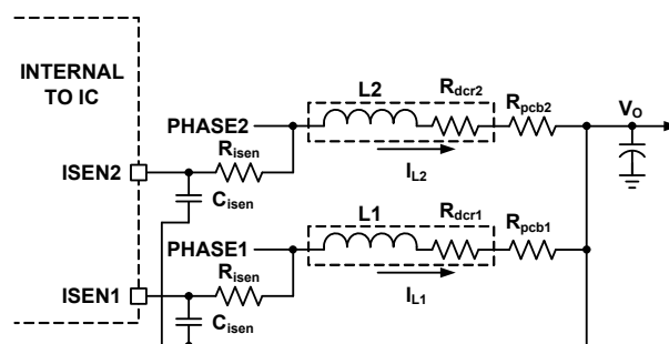
FIGURE 15. CURRENT BALANCING CIRCUIT
