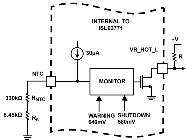
FIGURE 31. THERMAL MONITOR FEATURE OF THE ISL62771
