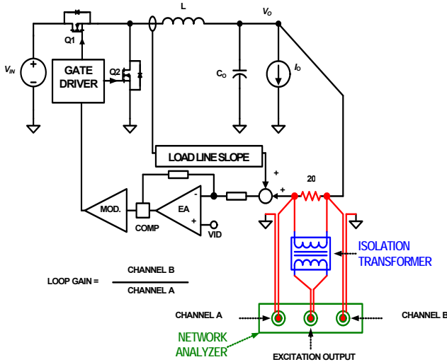
FIGURE 30. LOOP GAIN T2(s) MEASUREMENT SET-UP
