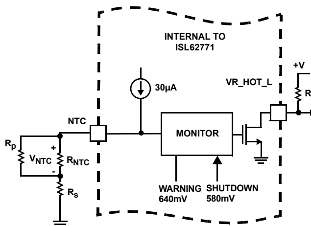
FIGURE 19. CIRCUITRY ASSOCIATED WITH THE THERMAL MONITOR FEATURE OF THE ISL62771
