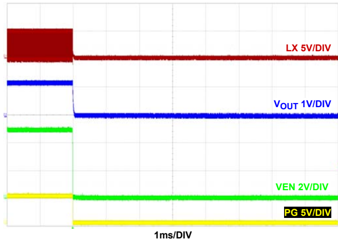
FIGURE 26. SHUTDOWN AT 2A LOAD F_{SW} = 2\text{MHz} , V_{IN} = 5\text{V} , MODE = PWM, T_A = +25^\circ\text{C}
