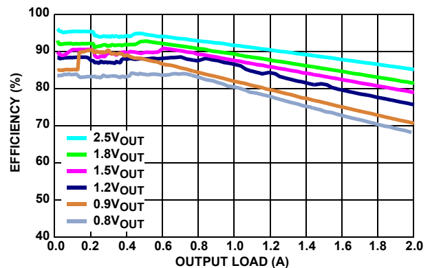
FIGURE 2. EFFICIENCY vs LOAD F_{SW} = 1\text{MHz} , V_{IN} = 3.3\text{V} , MODE = PFM, T_A = +25^\circ\text{C}
