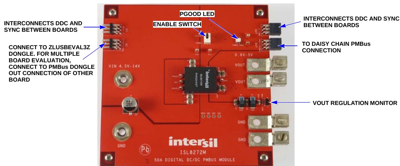
FIGURE 1. TOP SIDE
