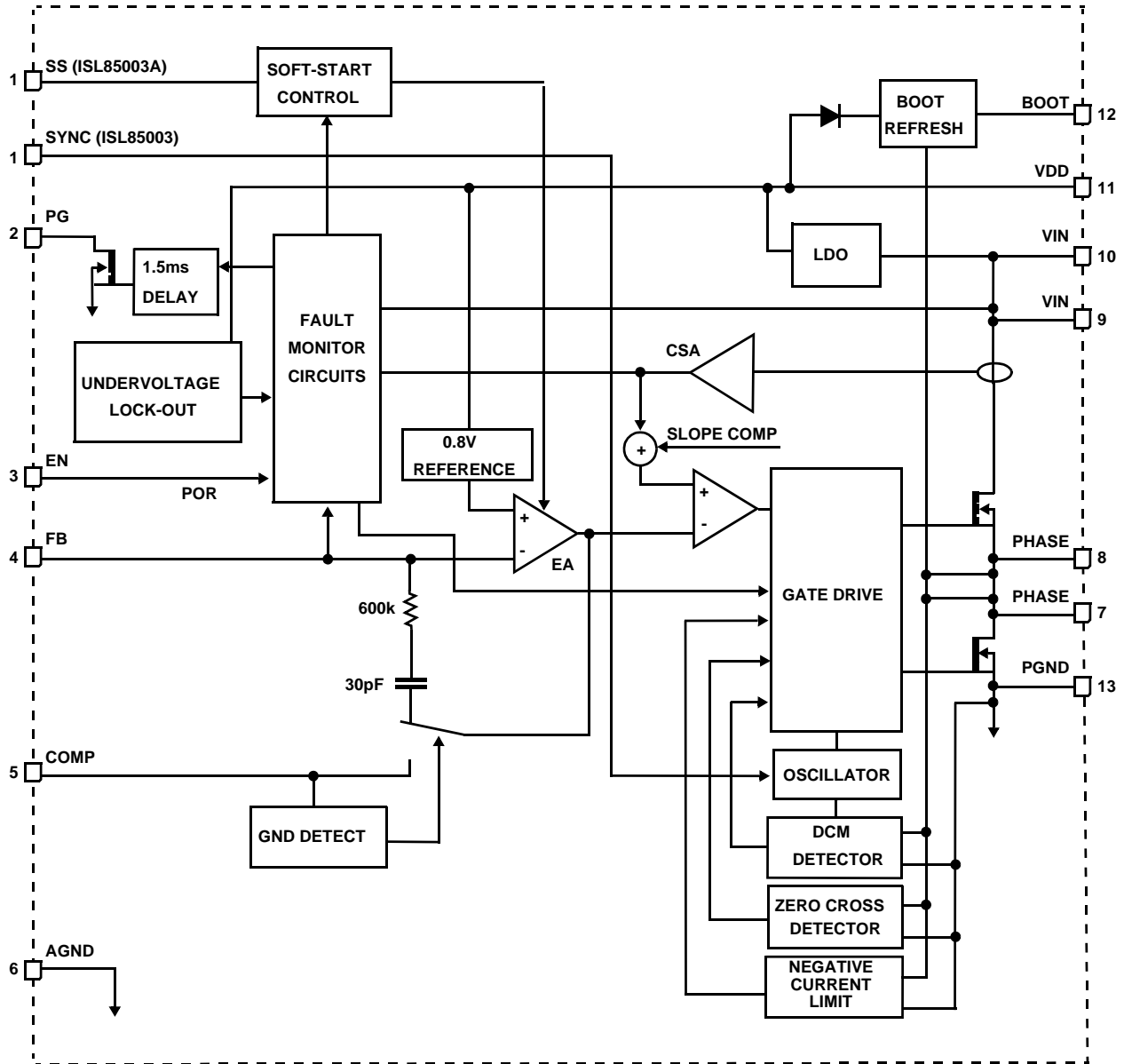
FIGURE 2. BLOCK DIAGRAM
