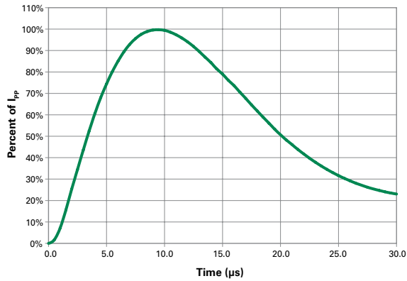
Pulse Waveform
