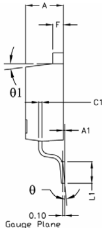
SIDE VIEW 1
