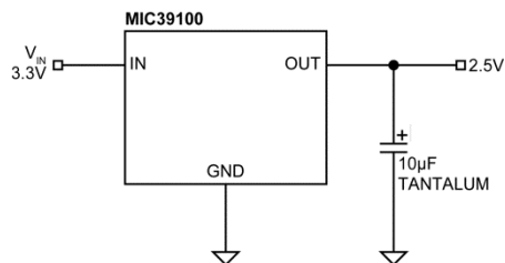
2.5V/1A Regulator
