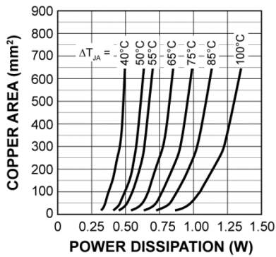
Figure 4. Copper Area vs. Power SOIC Power Dissipation ( \Delta T_{JA} )
