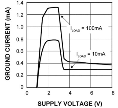
Ground Current vs. Supply Voltage (3.3V)
