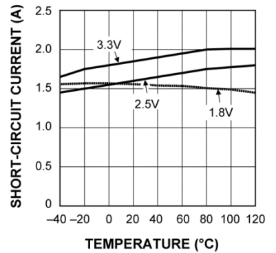
Short Circuit vs. Temperature
