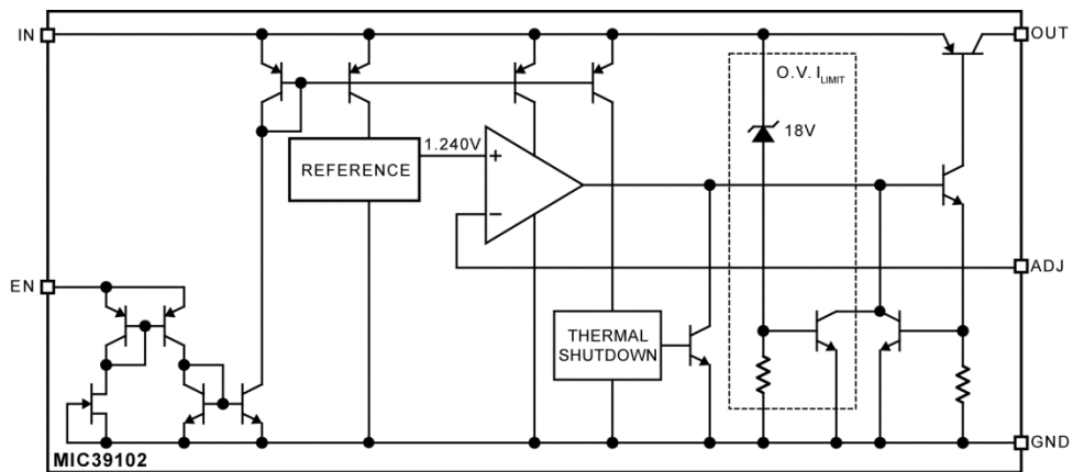
MIC39102 Adjustable Regulator Block Diagram
