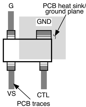
Figure 4. Heat-Sink Plane
