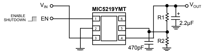
Ultra-Low-Noise Regulator (Adjustable)
