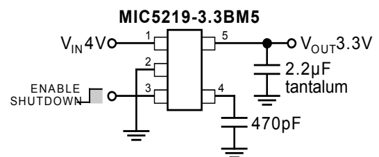
3.3V Ultra-Low-Noise Regulator
