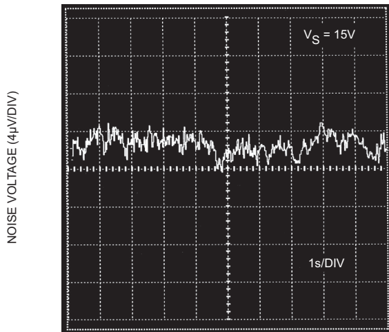
0.1Hz to 10Hz Noise
